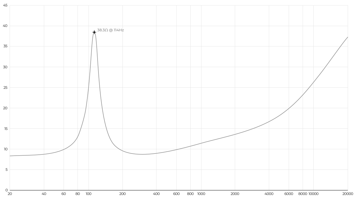
Torpedo Reload II Impedance Curve Measured at 8 \Omega
