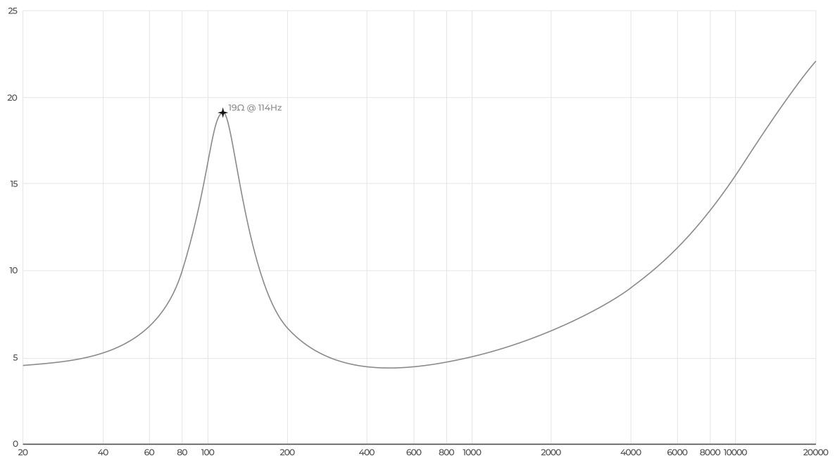
Torpedo Reload II Impedance Curve Measured at 4 \Omega
